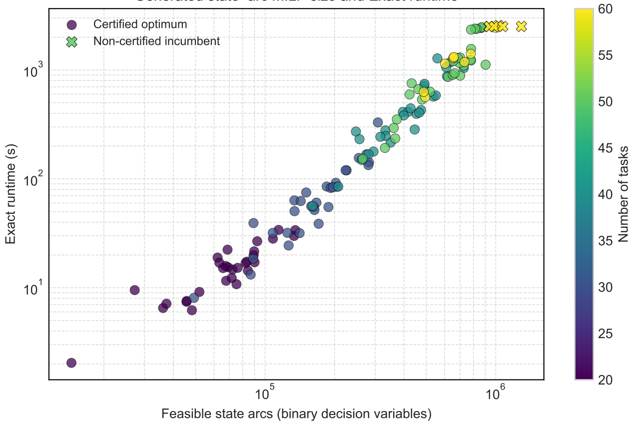
Generated state–arc MILP size and Exact runtime
